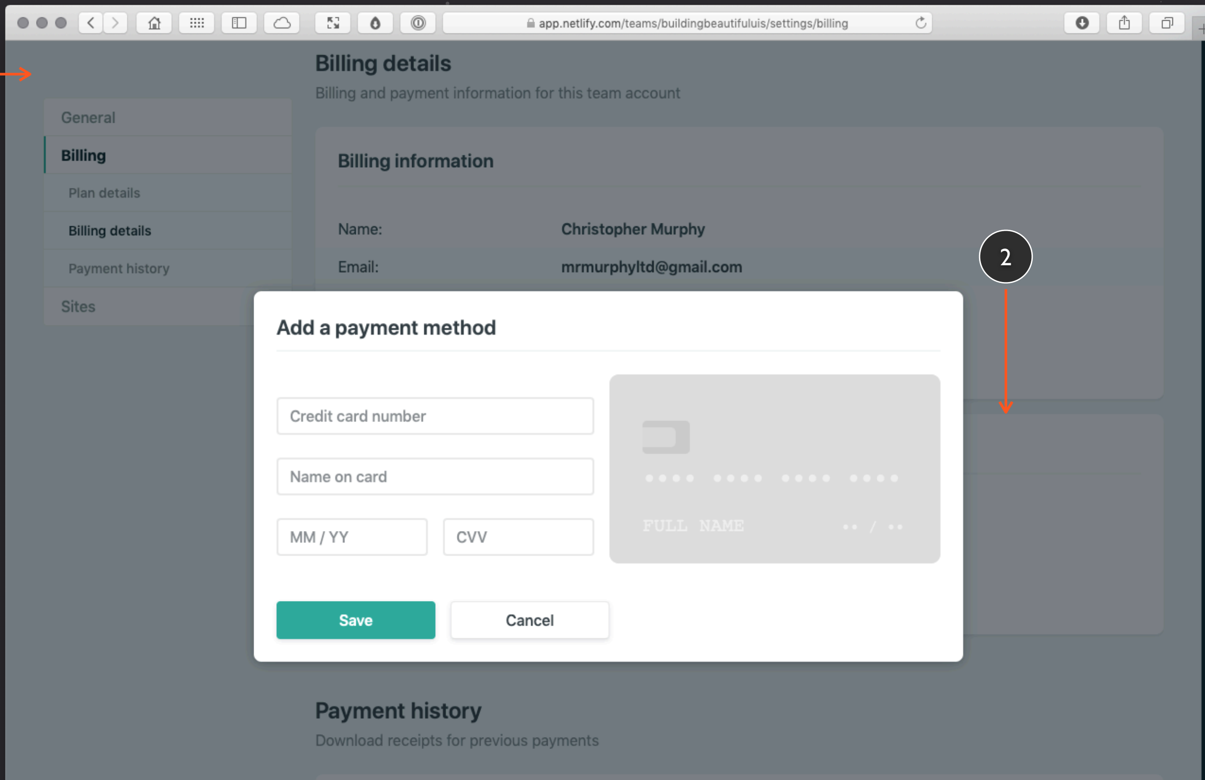
1. A grey overlay fades in. 2. The modal dialog animates in from top to bottom.
