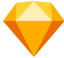
Sketch
