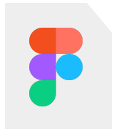
Figma file
