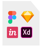
Design file
