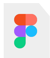
Figma file
