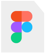
Figma file
