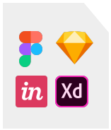
Design file
