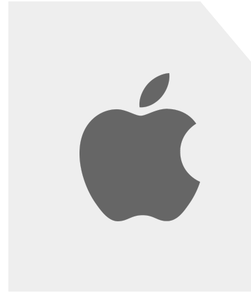
iOS
