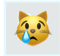
Photoshop
