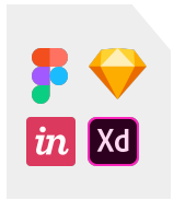
Design file
