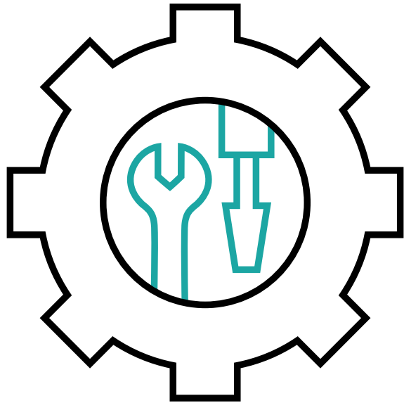
Production
