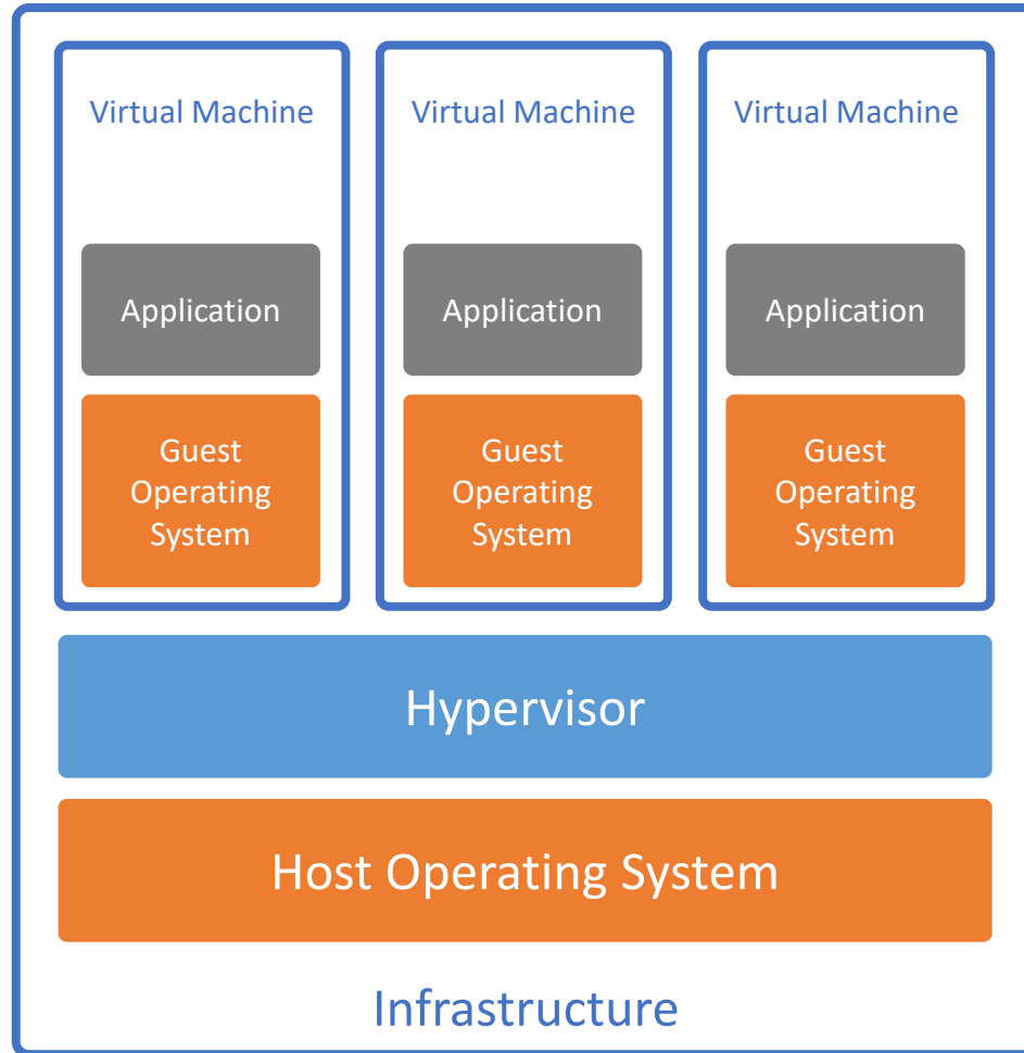
Virtual Machines
