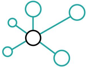
Dependencies
