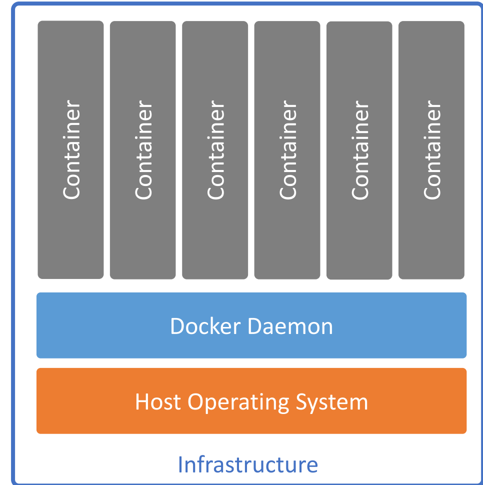
Containers
