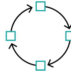
Environments
