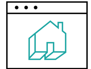
Operating Systems
