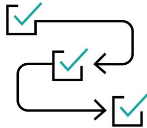
Deployments
