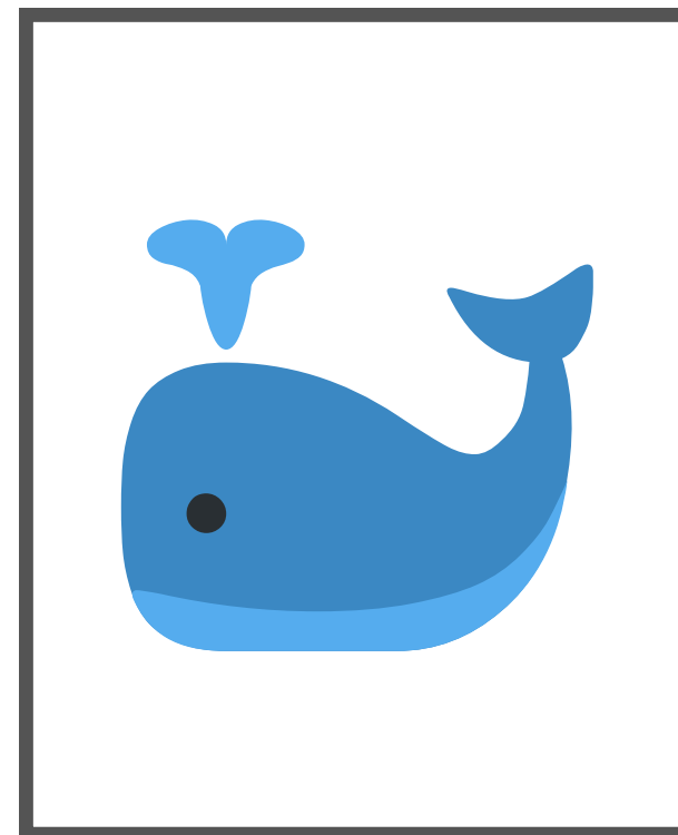
Docker Image
