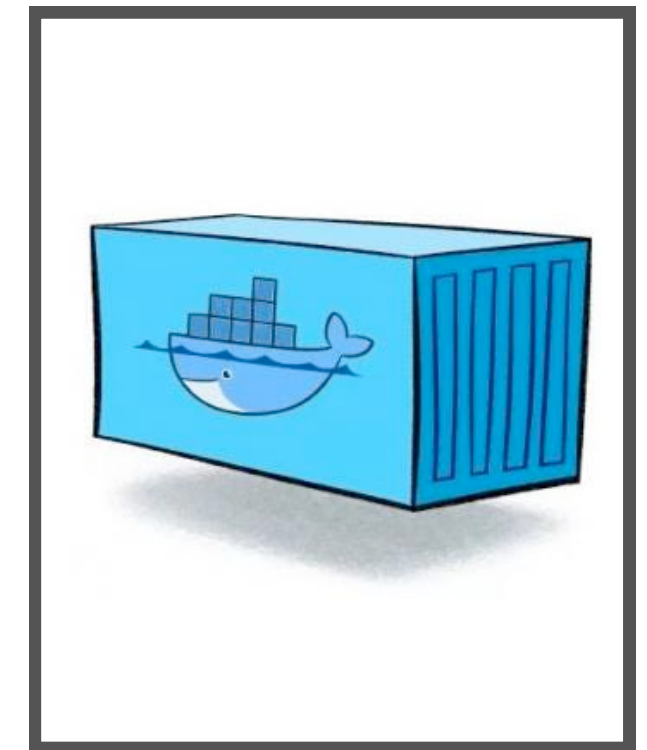
Docker Container
