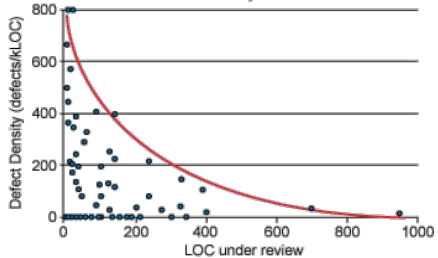
Defect Density vs. LOC
